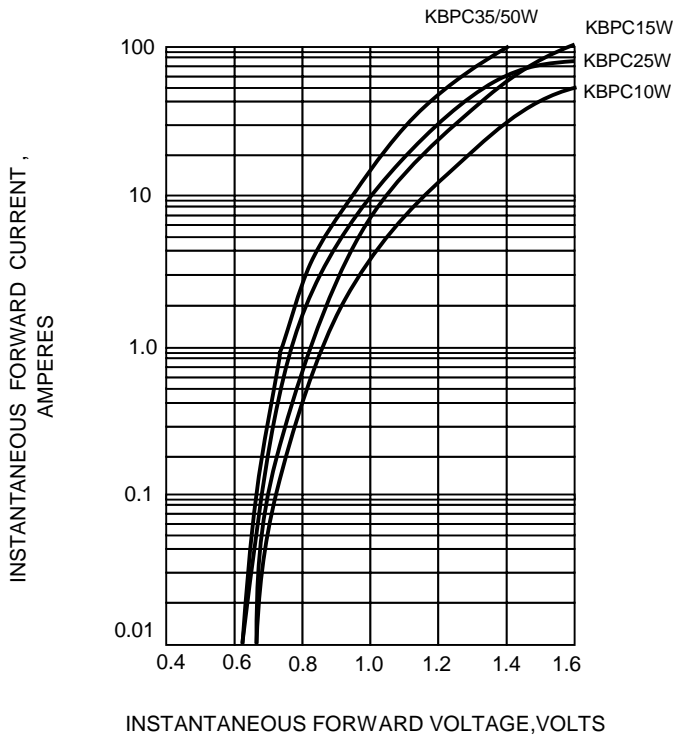
FIG.3-TYPICAL FORWARD CHARACTERISTICS
