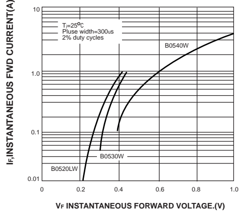
FIG. 2-TYPICAL FORWARD CHARACTERISTIC
