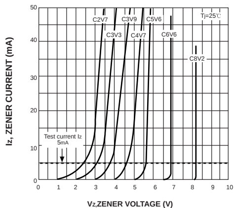
FIG. 2-ZENER BREAKDOWN CHARACTERISTICS
