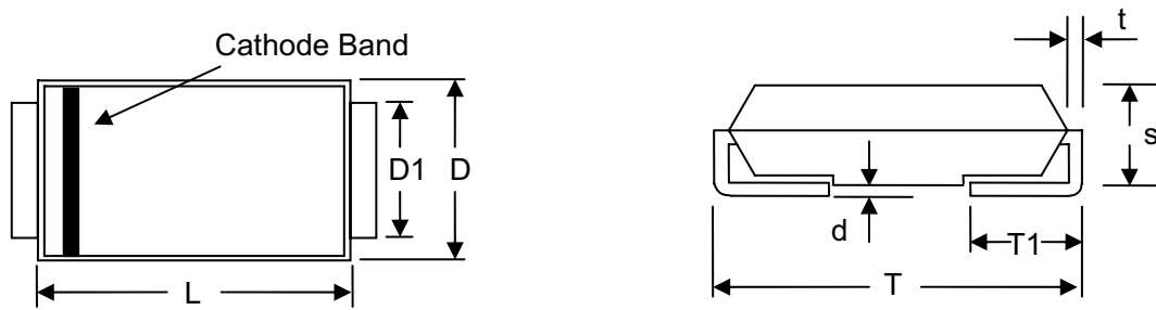
SMC/DO-214AB
